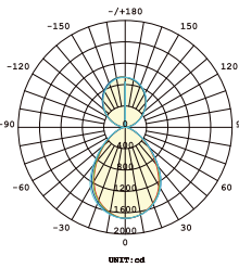
Photometric curves of SPACE 60 P-CL1500U-47W-840-80° ± 105° ↓
