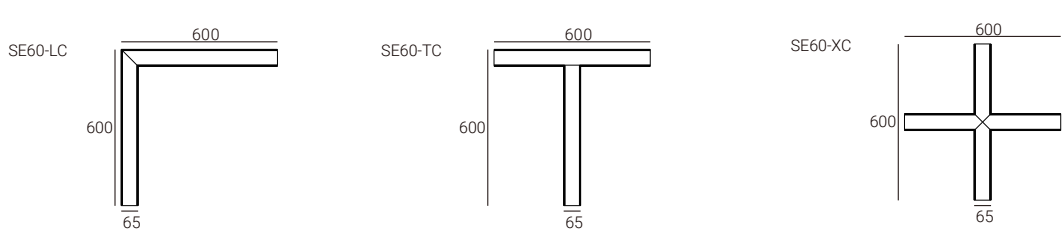
Corner Module of SPACE 60 Linear System
