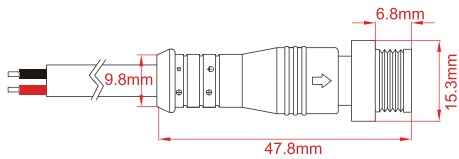
Male connector wire SYZ-M12-F-2C-075-W
